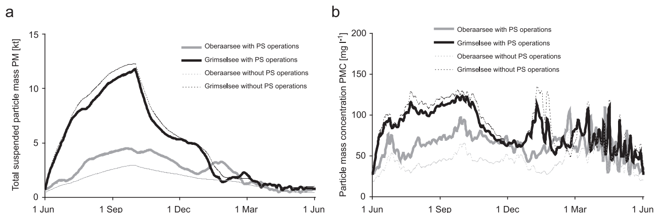
Figure 13. (a) One year simulation of volume-integrated suspended particle mass in Oberaarsee and Grimsensee, with and without PS operations. (b) One year simulation of PMC in Oberaarsee and Grimsensee, with and without PS operations. The variations in PMC in spring are due to the low water volume of the reservoirs and the corresponding large relative effect of particle input.
