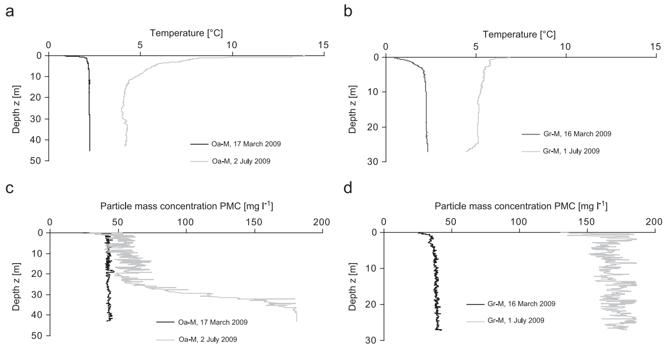
Figure 4. Temperature and PMC profiles in Oberaarsee and Grimselsee measured with a CTD in winter (16/17 March 2009; ice-covered; black lines) and in summer (1/2 July 2009; ice-free; gray lines) at the central reservoir locations Oa-M and Gr-M. (a) Oberaarsee temperature, with inverse stratification in winter and strong thermal stratification in summer. (b) Grimselsee temperature, with inverse stratification in winter and negligible stratification—compared to (Figure 4a)—in summer. (c) Oberaarsee PMC, with low surface PMC but high deep-water PMC in summer. (d) Grimselsee PMC, with also higher values in summer compared to winter and weak gradients with depth for both seasons.
