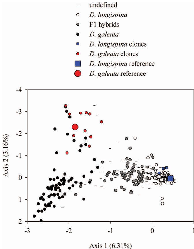
Fig. 5. Factorial correspondence analysis showing all genotypes from Fig. 4, but labeled by taxa determined by NewHybrids. Besides the two allozyme reference clones, additional D. galeata and D. longispina laboratory clones are shown. Undefined represents not significantly classifiable individuals.
