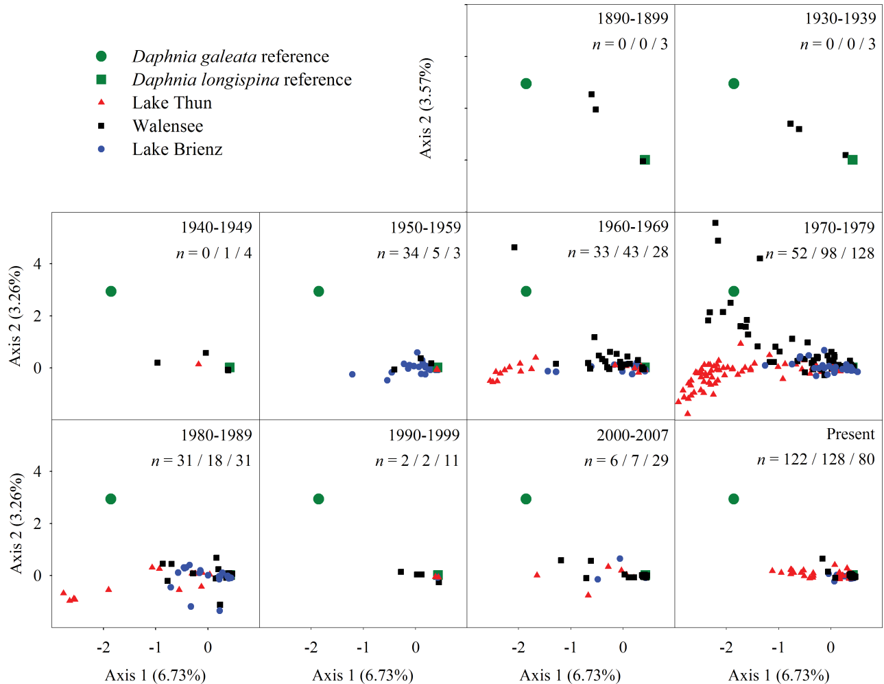
Fig. 4. Factorial correspondence analysis showing the past (diapausing eggs) and present (pelagic females) population structure of the three studied lakes during different decades. Allozyme reference clones for D. galeata and D. longispina are also included in the analysis. Each dot represents a genotype. Actual number of samples is also given (order: Lake Brienz/Lake Thun/Lake Walensee).
